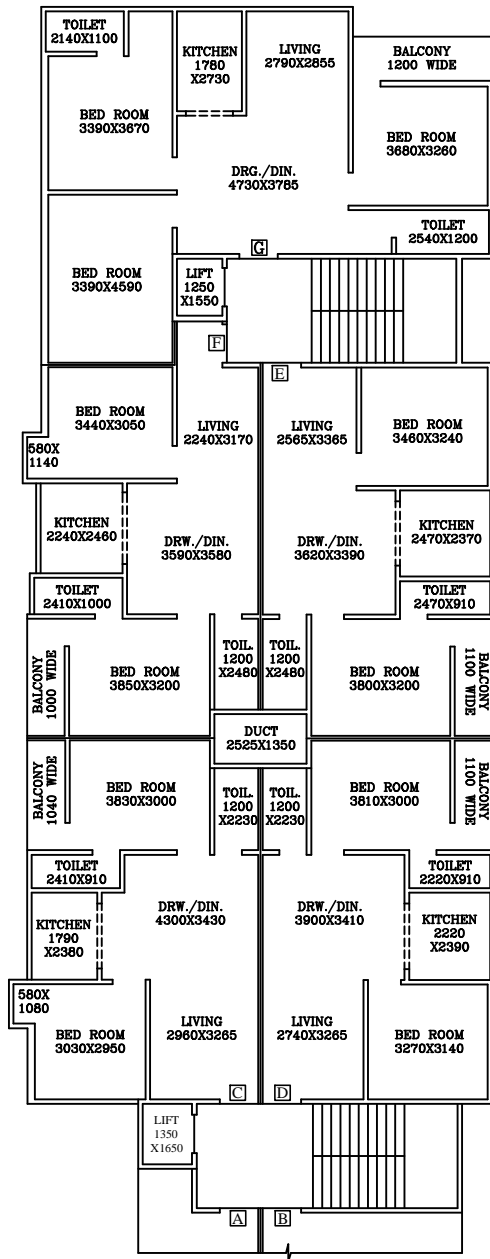
BLOCK-A FIRST FLOOR PLAN
