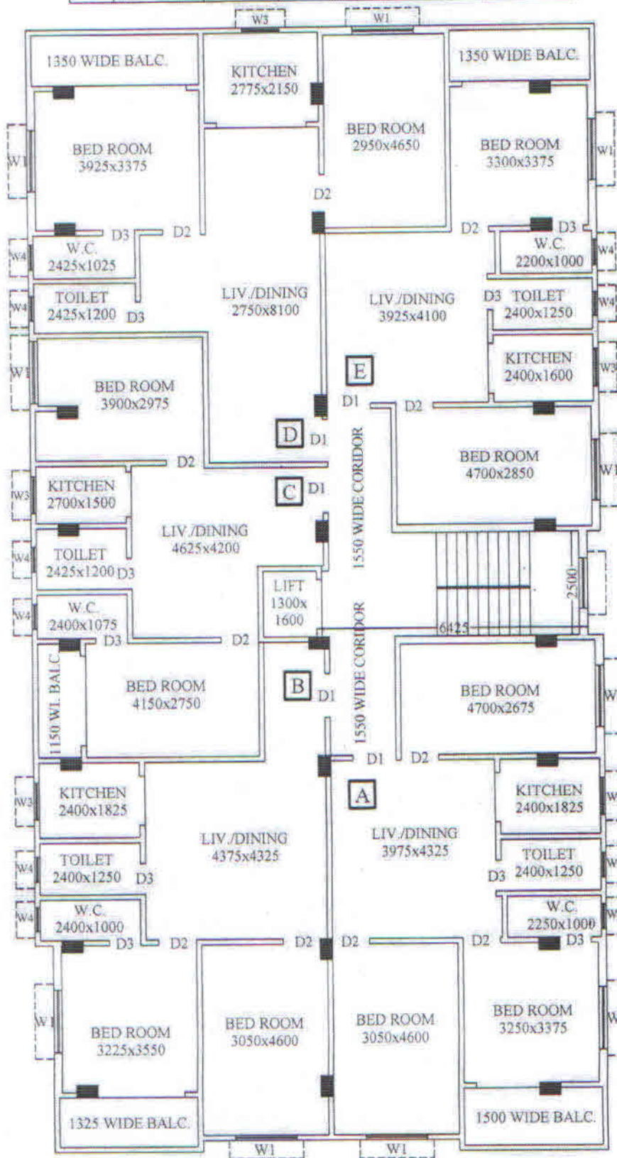
2ND, 3RD, 4TH & 5TH FLOOR PLAN (BLOCK- (B)) (TEEN PUKUR SITE)
