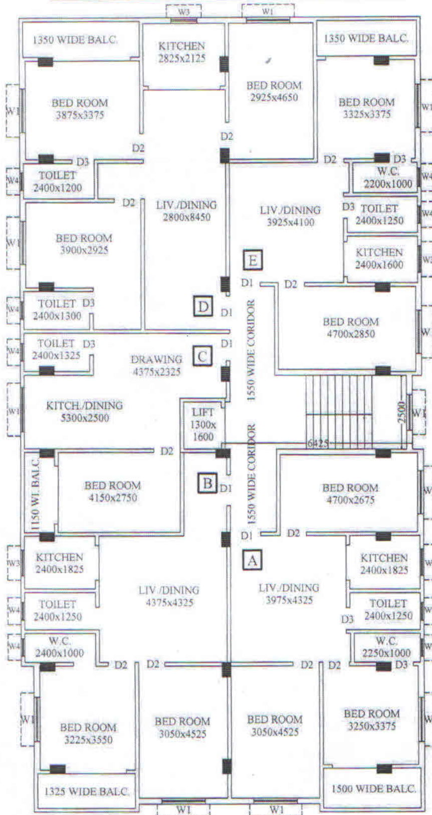
FIRST FLOOR PLAN (BLOCK- (B)) (TEEN PUKUR SITE)
