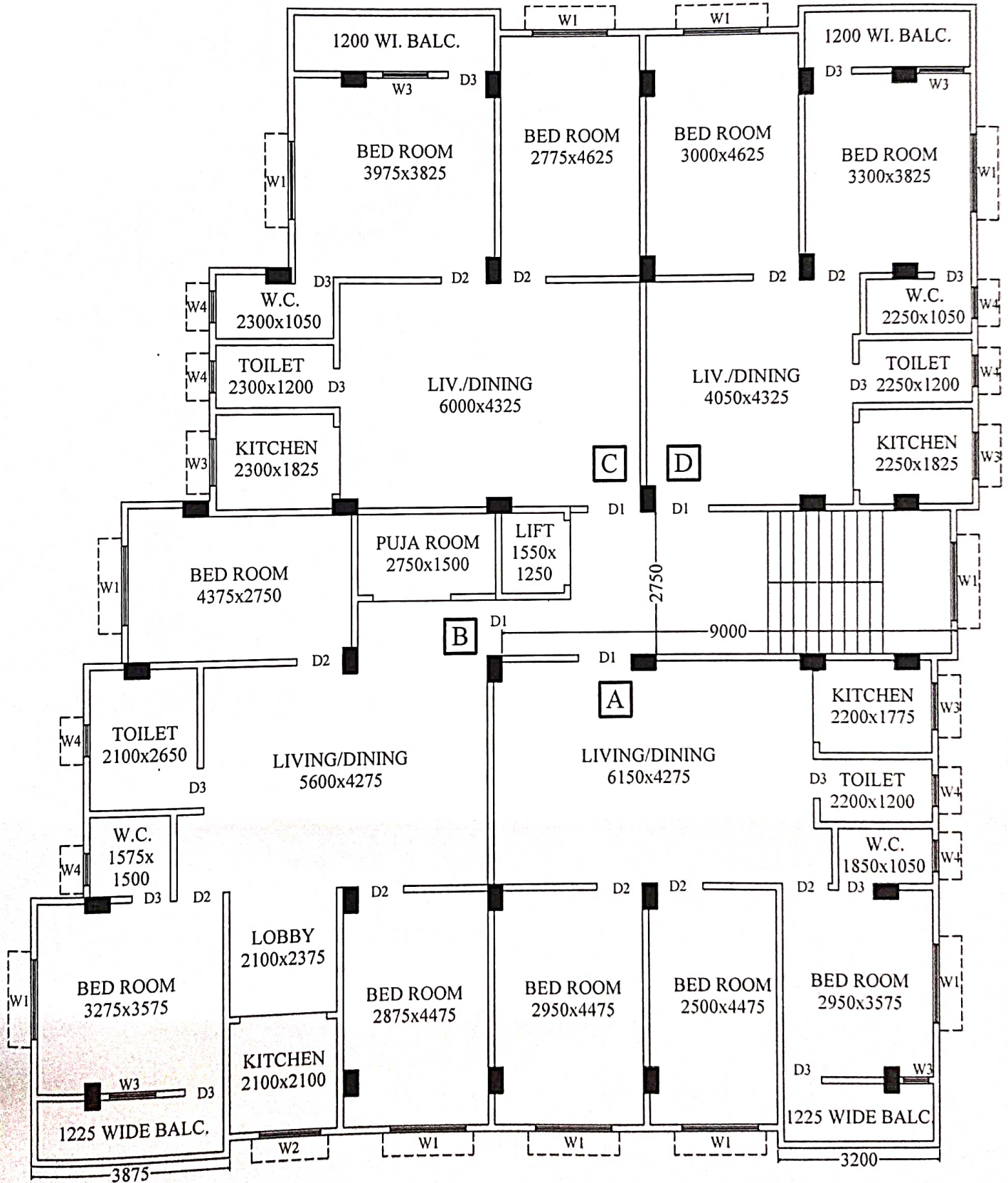
TYPICAL FLOOR PLAN (BLOCK- (A)) (TEEN PUKUR SITE)
